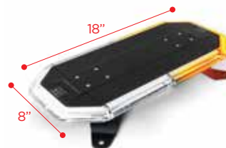
SLP1018AC / Permanent Mount
