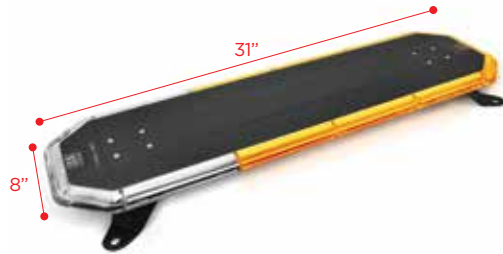
SLP 1030 / Permanent Mount
