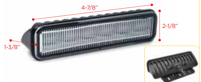
376A / 376AC 90° Degree Surface Mount
