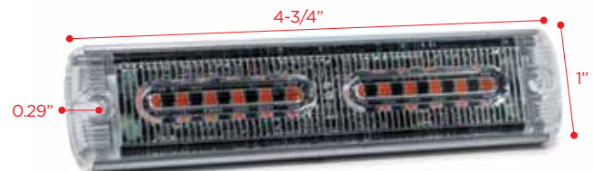
3675A / 3675AC Low Profile Surface Mount
