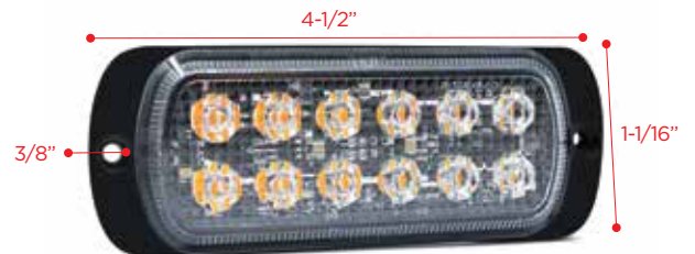
312A / 312AC Low Profile Surface Mount
