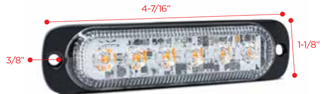
306A / 306AC Low Profile Surface Mount
